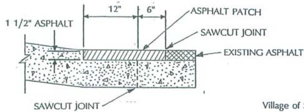
DRIVEWAY ON STREET
