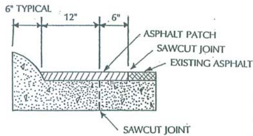
INTEGRAL CONCRETE CURB
