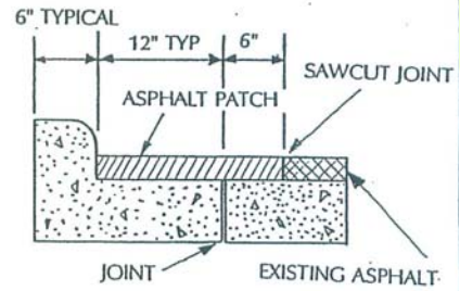
CONCRETE CURB AND GUTTER
